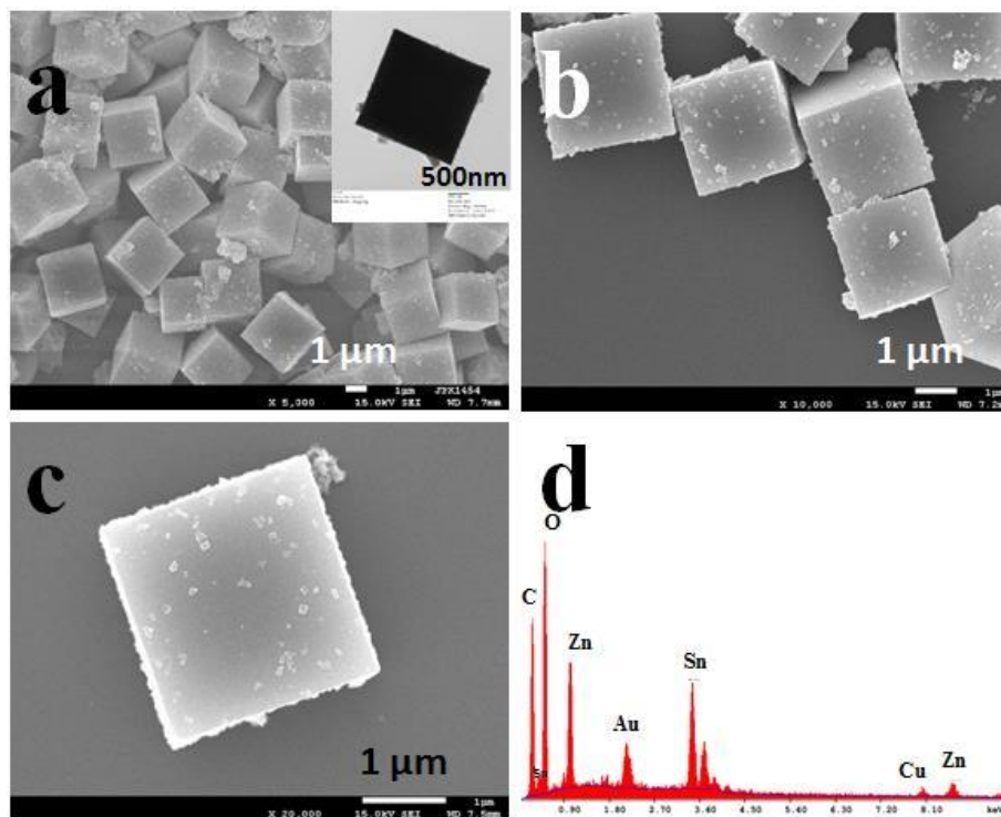
Figure 15: ZnSn(OH) 6 mesocubes: (a-c) FESEM images and (d) EDS of cubic ZnSn(OH) 6 precursor obtained at room temperature with 0.32M NaOH. Inset of (a) is the TEM image of cubic ZnSn(OH) 6 precursor
