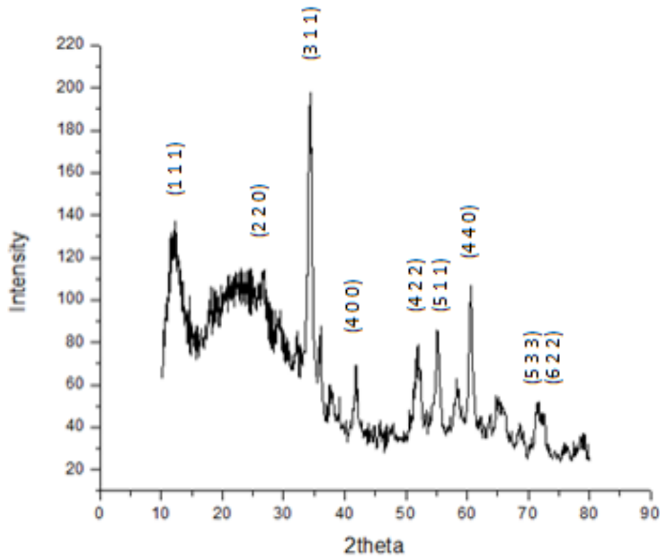
Figure 28: XRD pattern of Zn_2SnO_4/SnO_2
