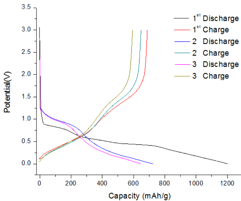
Figure 31: Discharge-charge curves of the electrode Zn 2 SnO 4 /SnO 2 .
